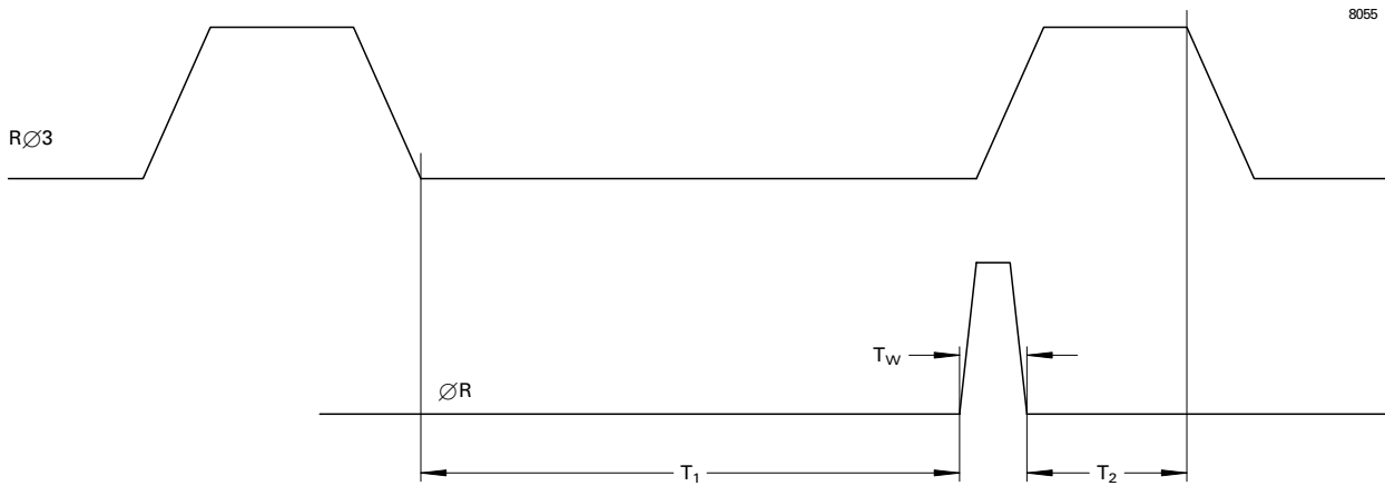
Figure 9: RESET PULSE
