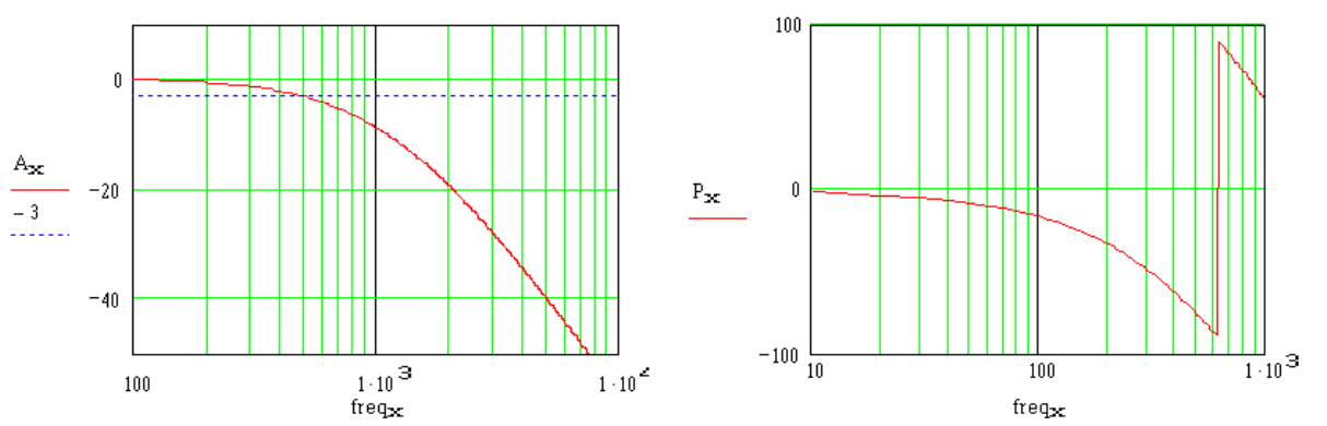
Figure 12: G100Z “LN Series” Frequency Response
