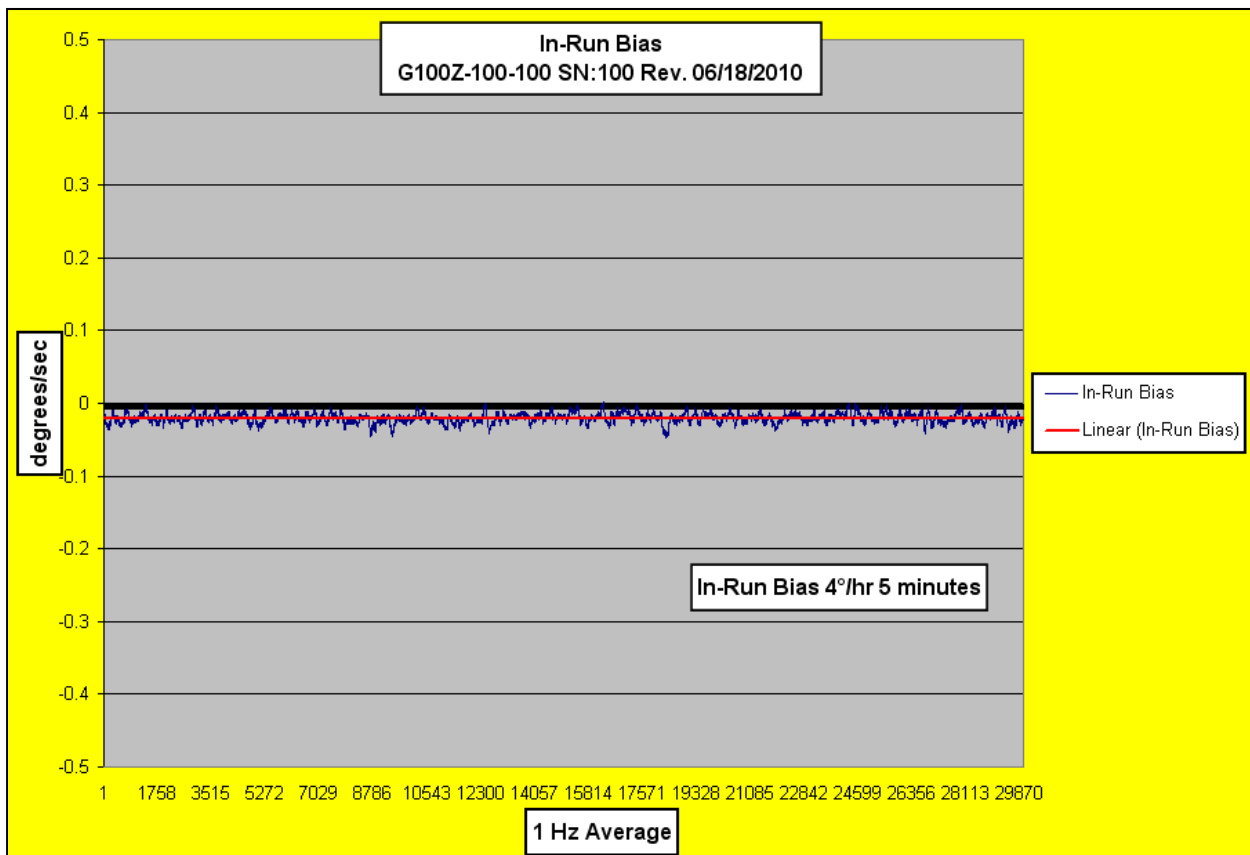
Figure 15: In-Run for G100Z-100-100 SN: 100
