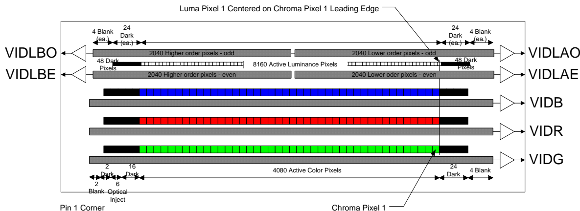
Figure 1: Block Diagram
