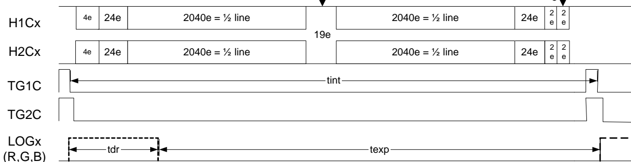
Figure 17: Line Timing Diagram
