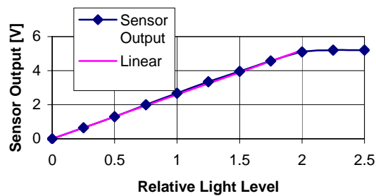
Figure 10: KLI-8023 Typical Device Response Linearity
