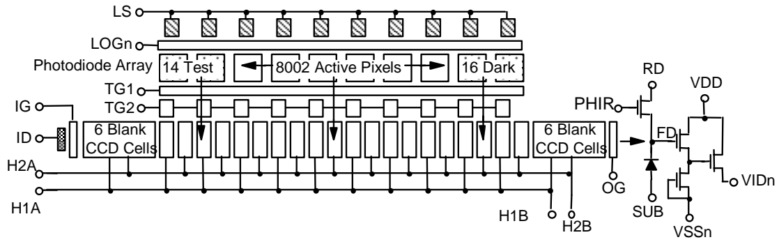
Figure 1: Single Channel Schematic
