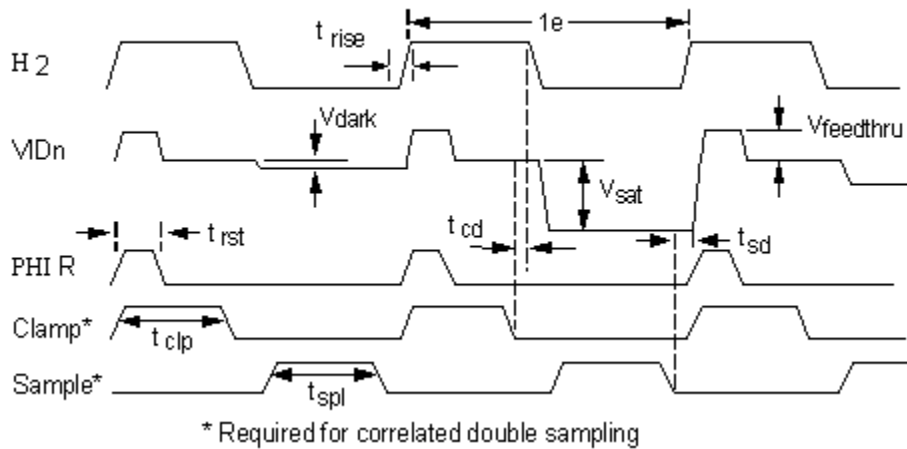
Figure 14: Output Timing
