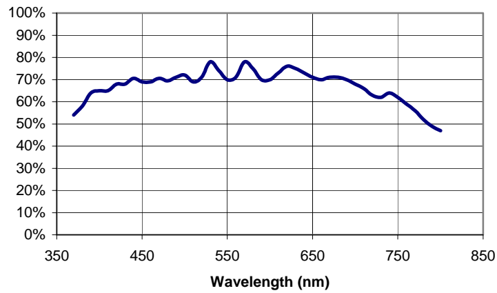
Figure 4: KLI-8023 (monochrome) Typical Quantum Efficiency (%)
