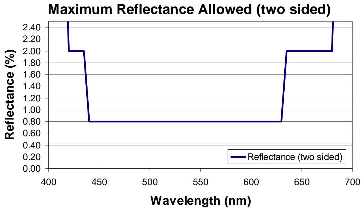
Figure 17: Two-Sided Multilayer Anti-Reflective Cover Glass Specification (MAR)
