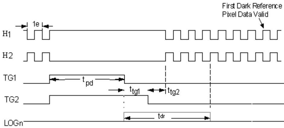
Figure 13: Photodiode-to-CCD Transfer
