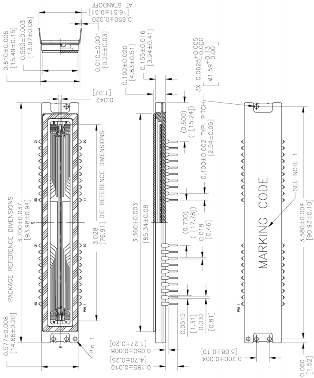
Figure 15: Completed Assembly Drawing (1 of 2)
