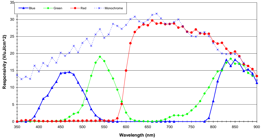
Figure 2: KLI-8023 Typical Responsivity
