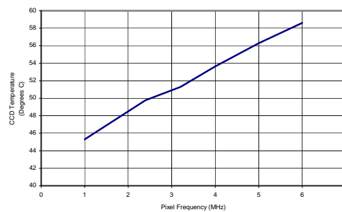
Figure 9: KLI-8023 Typical CCD Temperature Vs. Operating Frequency
