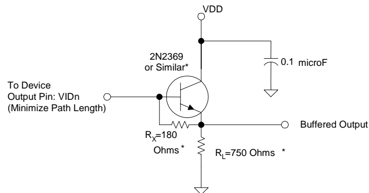
Figure 11: Typical Output Bias/Buffer Circuit
