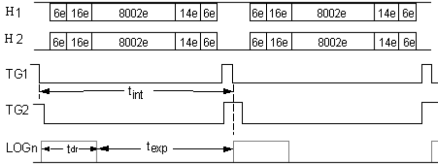
Figure 12: Line Timing
