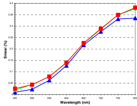
Figure 5: KLI-8023 Smear - LDR Operation / 1 MHz / 35 C
