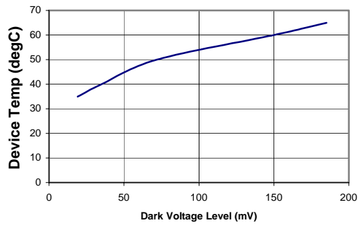
Figure 8: KLI-8023 Typical Dark Pixel Voltage Level vs. Temperature
