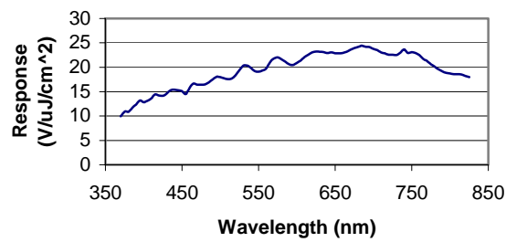
Figure 6: Monochrome KLI-8023 Spectral Response
