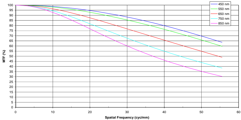
Figure 3: KLI-8023 Typical Modulation Transfer Function
